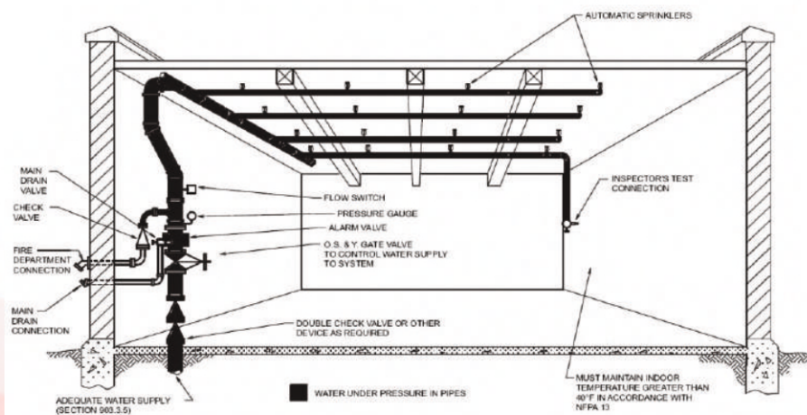
Schematic Drawing of Fire Sprinkler System
