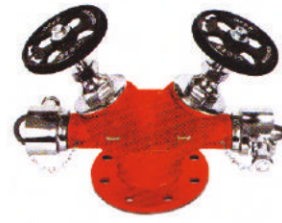
Landing Valve
