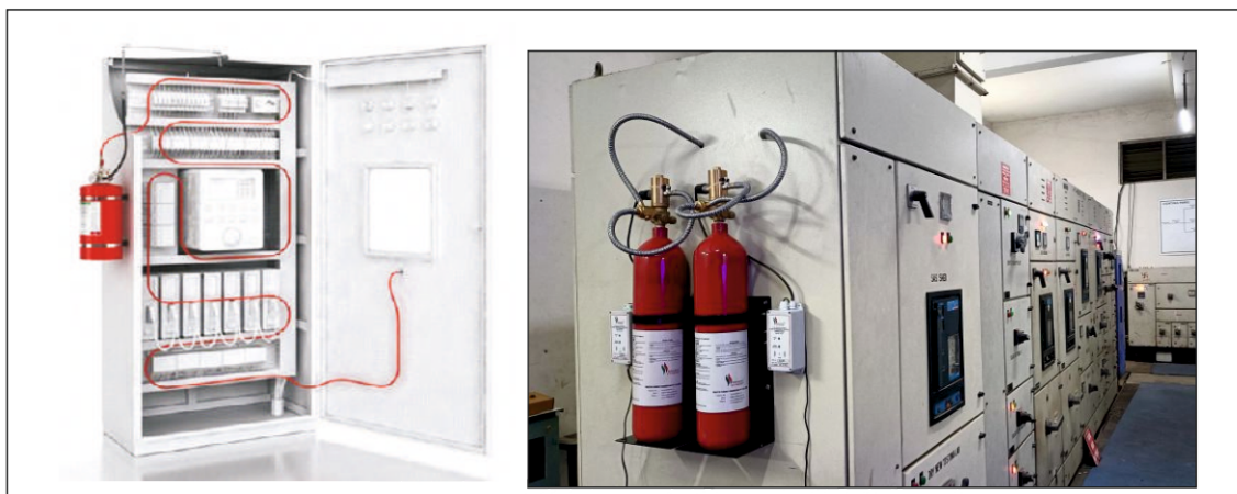
Fire Suppression System For Electrical Panel
