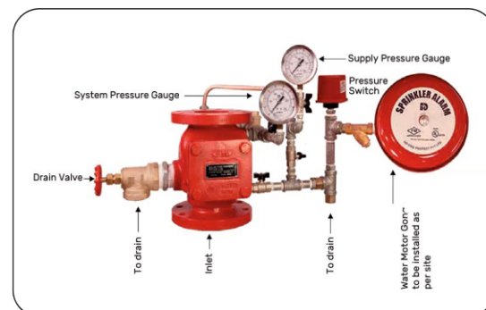
Sprinkler Alarm Valve
